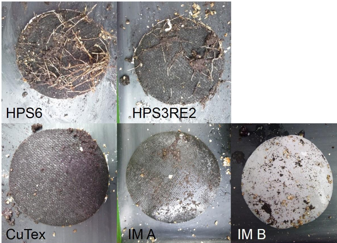
Figure 4: Example photographs of the under-side of specimens, showing presence or absence of lupin root penetration through the specimen.
